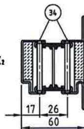
Detail X 2
